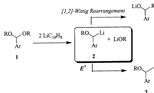
Scheme 1. Reduction of aromatic acetals
